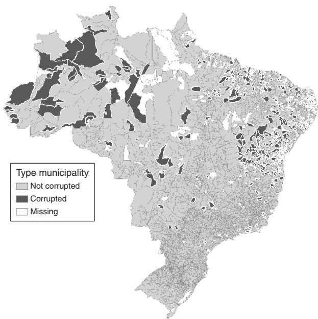
FIGURE 3. THE GEOGRAPHY OF (PREDICTED) CORRUPTION
