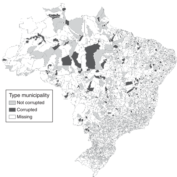
Panel B. Predicted corruption
