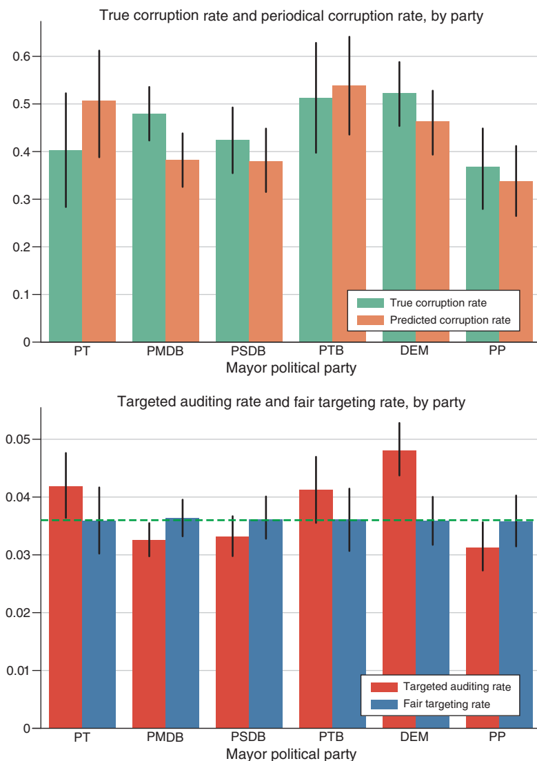
FIGURE 5. CORRUPTION RISK AND TARGETED AUDITING, BY PARTY
