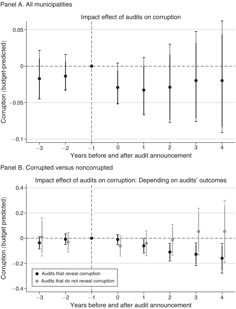
FIGURE 4. DYNAMIC EFFECT OF AUDITS ON FISCAL CORRUPTION
